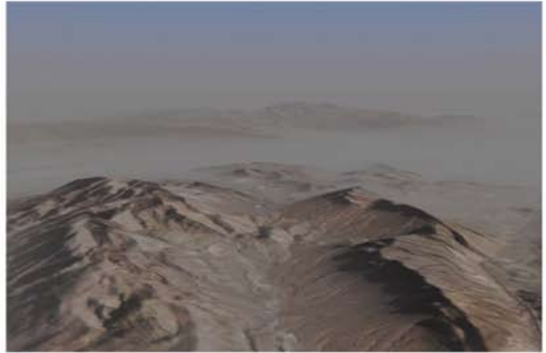
Ground Fog with Haze
