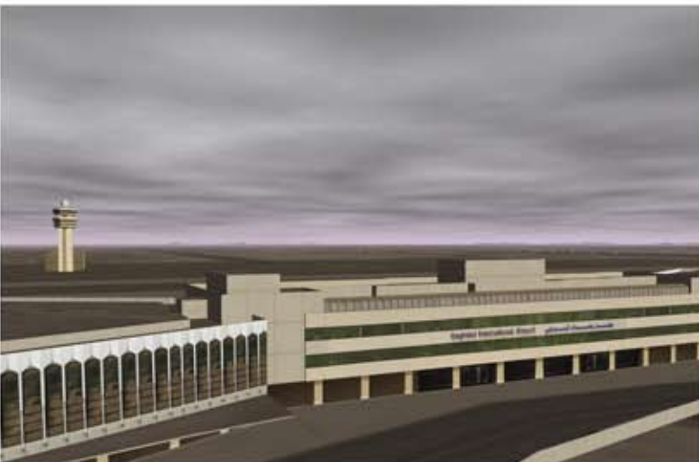
Low Cloud Deck with Haze
